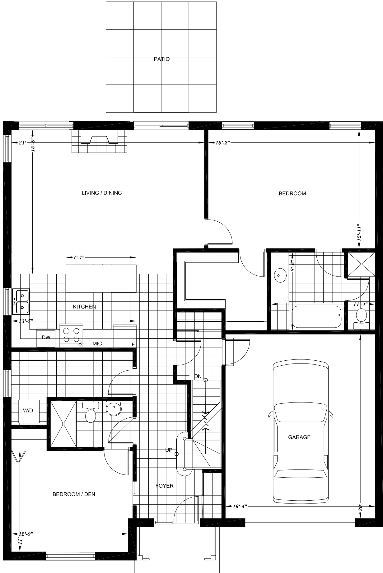
Main Floor - 1505 sq.ft.
