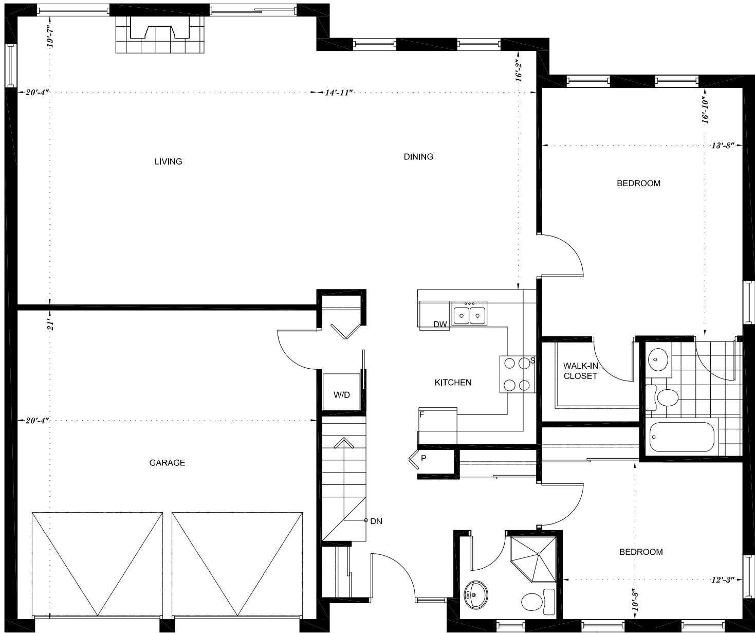
Main Floor - 1587 sq.ft.
